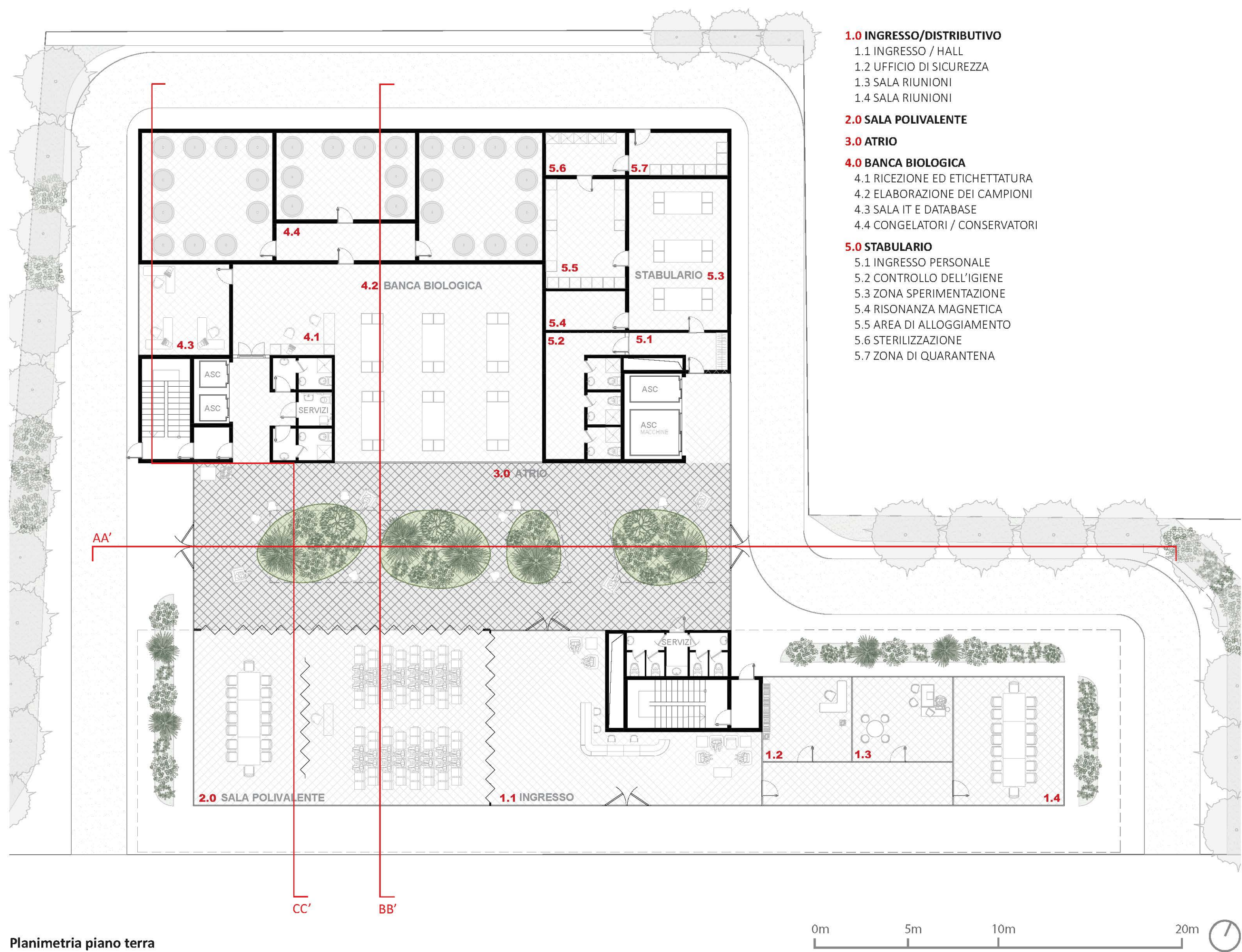
Planimetria piano terra
