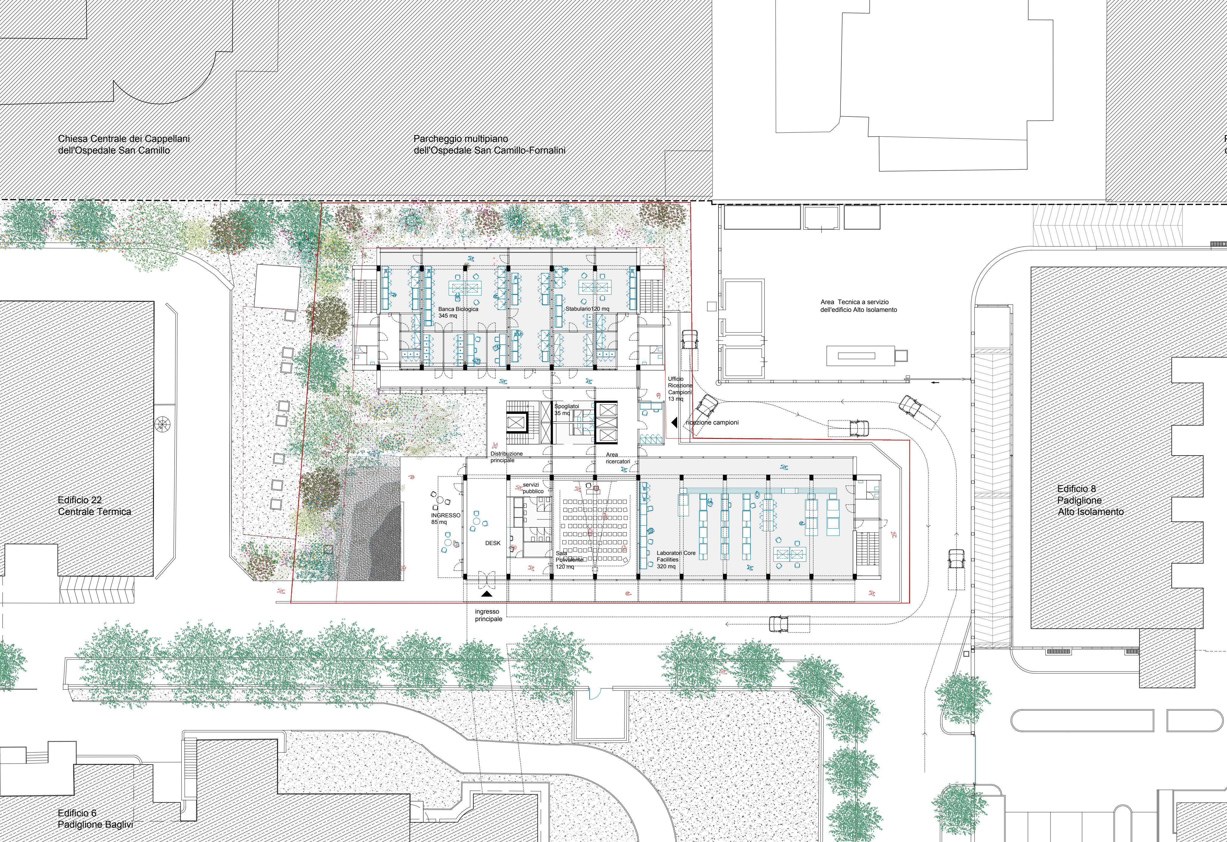
PLANIMETRIA PIANO TERRA SCALA 1:250
