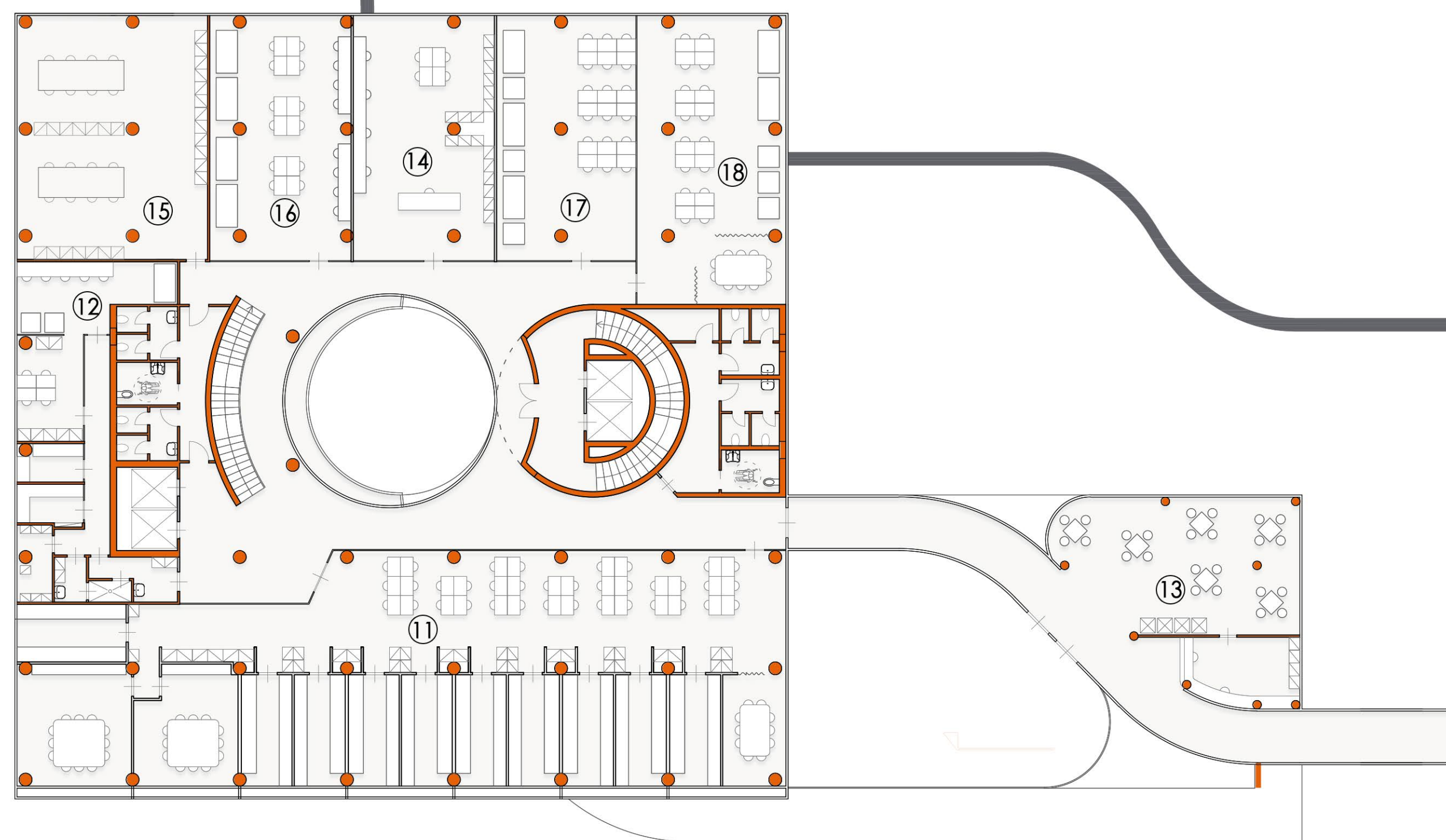
PIANO 2 ▼ + 08.75
