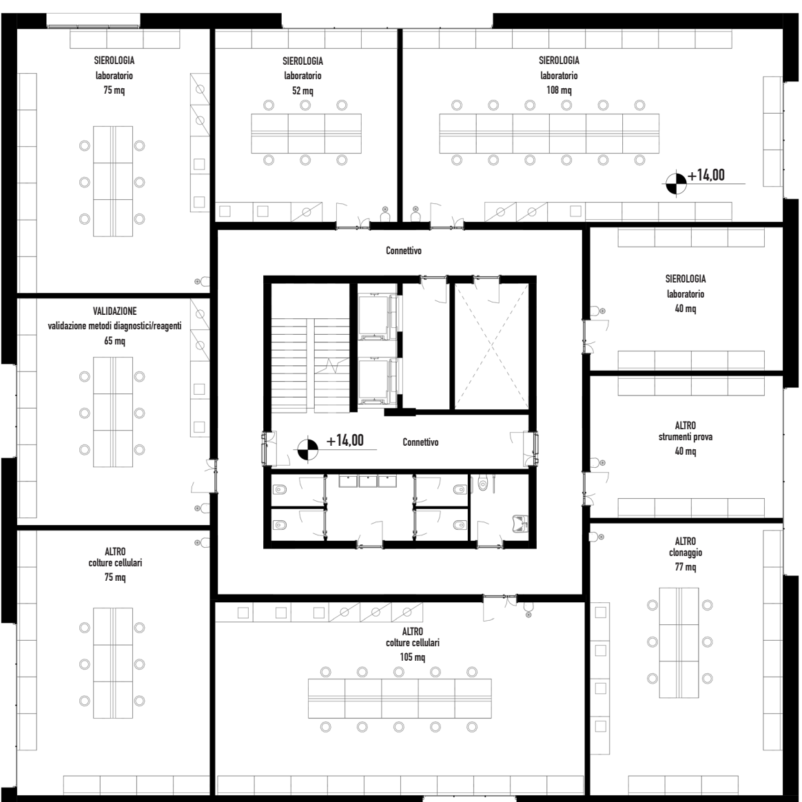
PIANO QUARTO 1:200 (+14,00)
