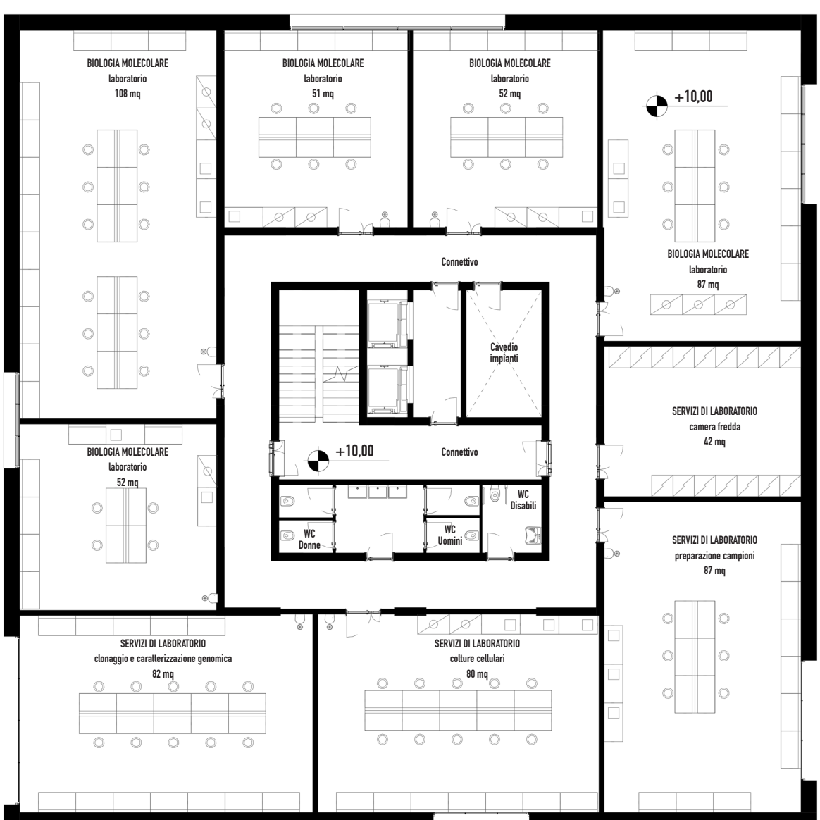
PIANO TERZO 1:200 (+10,00)
